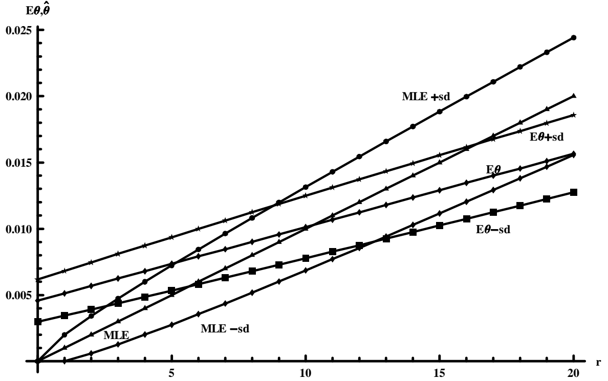
Figure 6: E\theta and MLE \hat{\theta} for n=1000
