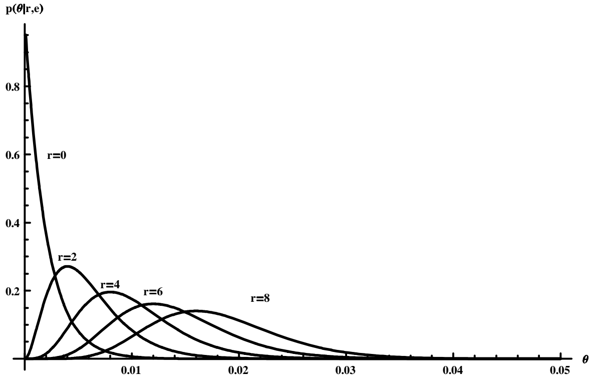
Figure 1: Likelihood Functions n=500
