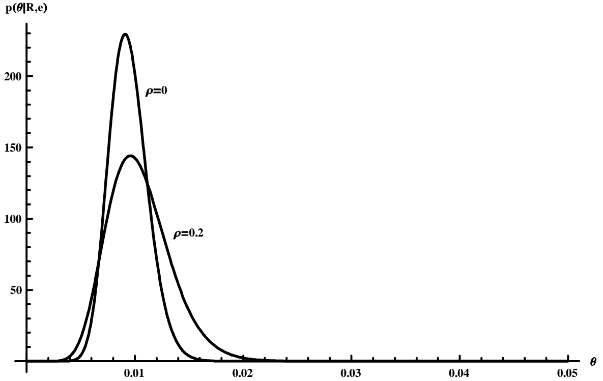
Figure 9: Posterior with Heterogeneity
