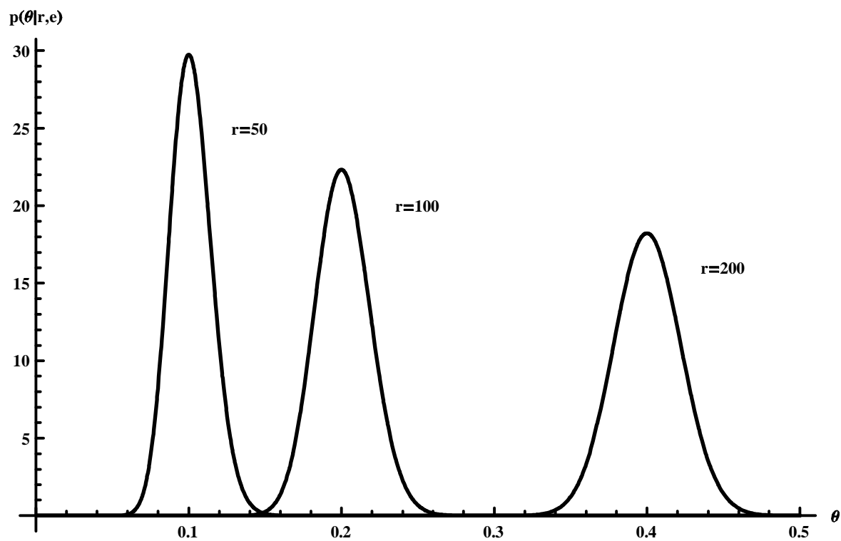
Figure 8: Posteriors with \epsilon=0.01 , n=500
