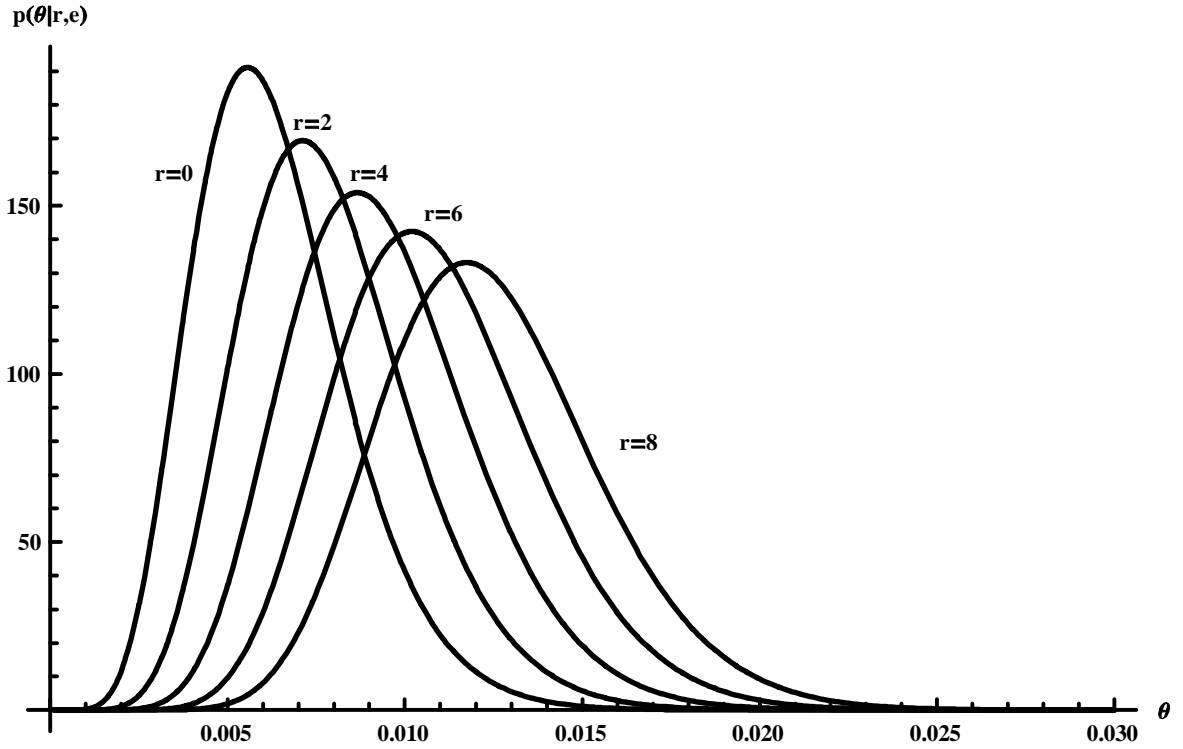
Figure 5: Posterior Densities p(\theta|r,e)
