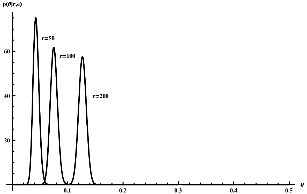
Figure 7: Posteriors with \epsilon=0 , n=500
