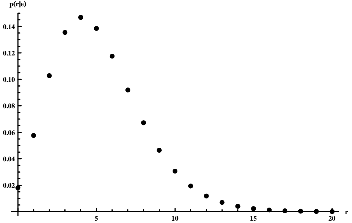
Figure 4: Predictive Distribution p(r|e)
